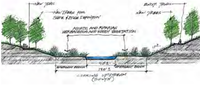
Image 5. Channel cross-section illustrating proposed improvements, Image Source: Union-Oxford South Platte River Rehabilitation & Recreation Improvements by McLaughlin Whitewater Design Group, March 2013.
